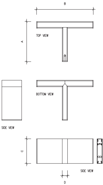
BX-1-T Connector
