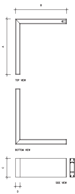
BX-1-L Connector
