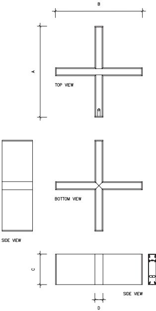
BX-1-X Connector
