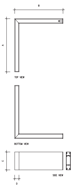
BX-1-L Connector
