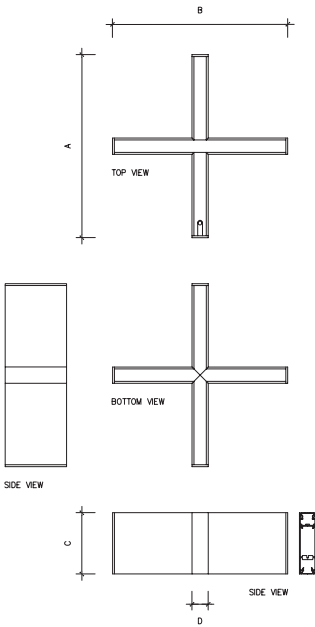
BX-1-X Connector
